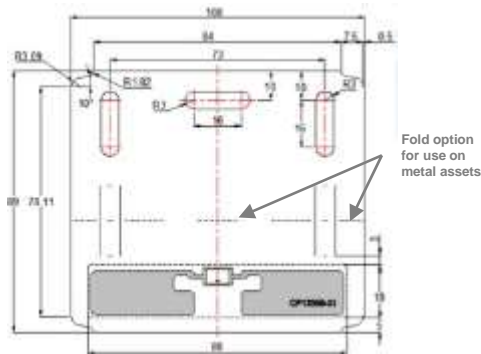
The IQ 1200P hang tag includes a flag feature (fold out inlay) option, to optimize the capability to tag metallic assets.
