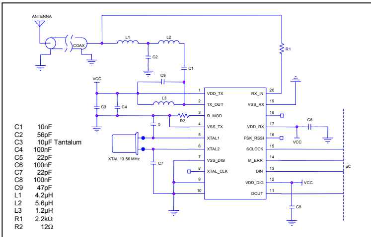
Recommended application schematic
